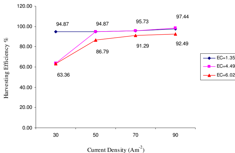
Figure 5. Effect of EC on harvesting efficiency at three different EC.
