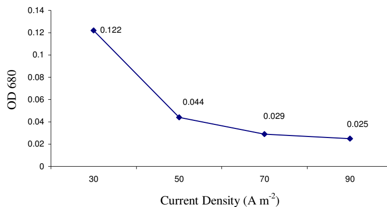
Figure 2. Decreasing of OD_{680} by increase in current density at EC = 6.02 \text{ S m}^{-1} .
