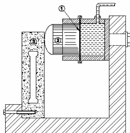
Figure 3. A schematic diagram of the force magnifying piston and cylinder, showing the locations of the elastic membrane (1), piston (2) and strain gage load cell (3).
