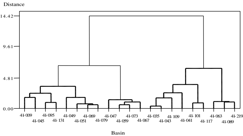
Figure 2. Dendrogram of clustered basins by Ward’s method.
