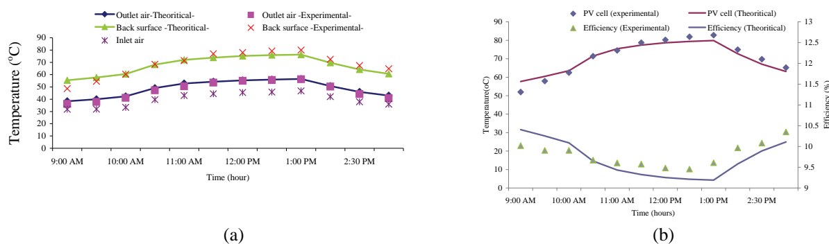
Figure 4. (a) Hourly variation of inlet air temperature and experimental validation of outlet air temperature back surface temperature for the glass to tedlar PV/T solar collector, (b) Experimental validation of the solar cell temperature and electrical efficiency for the glass to tedlar PV/T solar collector.
