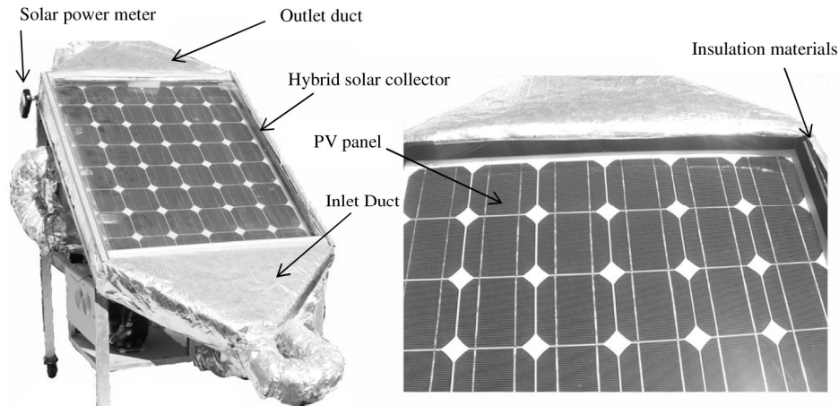
Figure 2. (a) Photograph of the experimental setup of hybrid PV/T solar collector and (b) Close view to the two-way PV/T solar collector structure.
