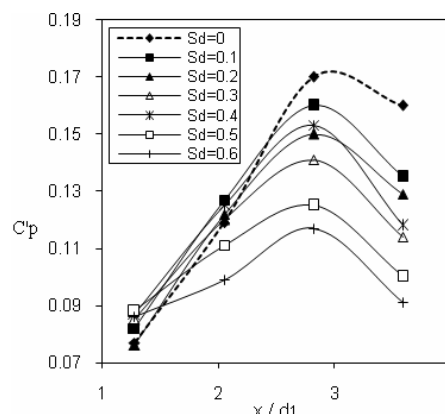
Figure 9. Variation of C'_p with S_d at XZ-plane and elevation of Z= H/8 from the top face in X- direction for Fr_1= 7 .
