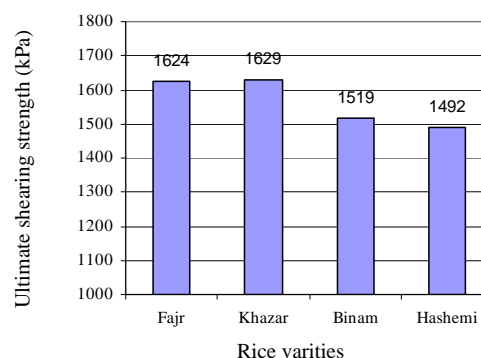
Figure 3. Static ultimate cutting force for four varieties.
