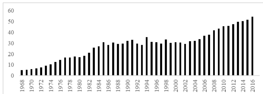
Figure 3. Agricultural energy consumption (Million barrels of oil equivalent). Source: Iran's Ministry of Energy.
