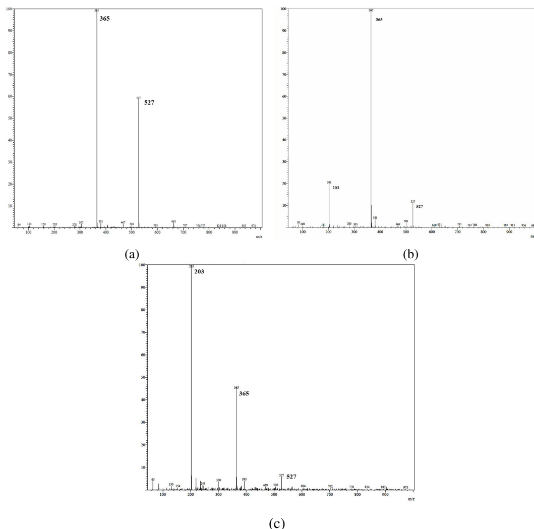
Figure 2. Mass spectrogram of the fractions pooled from gel chromatography as shown in Figure 1. (a) The fraction of the 11 th to the 14 th tubes; (b) The fraction of the 15 th to the 17 th tubes, and (c) The fraction of the 18 th to the 19 th tubes.
