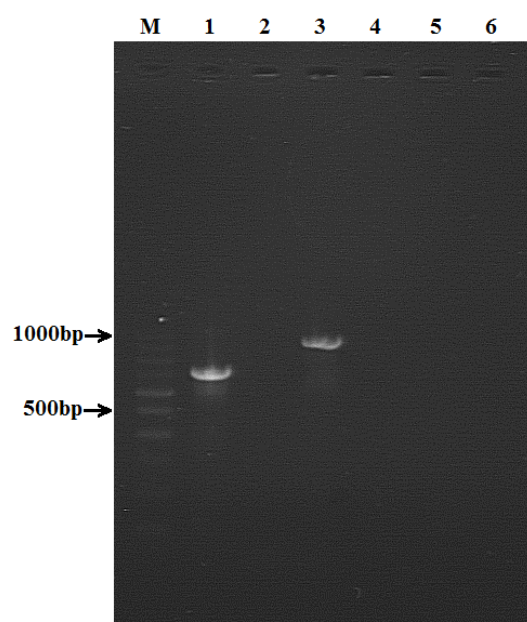
Figure 1. Diagnostic PCR using species-specific primers. Lane M: DNA size marker; Lane 1: T. urticae DNA+UrtF primer; Lane 2: T. urticae DNA+TurkF primer, Lane 3: T. turkestan i DNA+TurkF primer; Lane 4: T. turkestan i DNA+UrtF primer; Lane 5: C - (with UrtF primer), Lane 6: C - (with TurkF primer).
