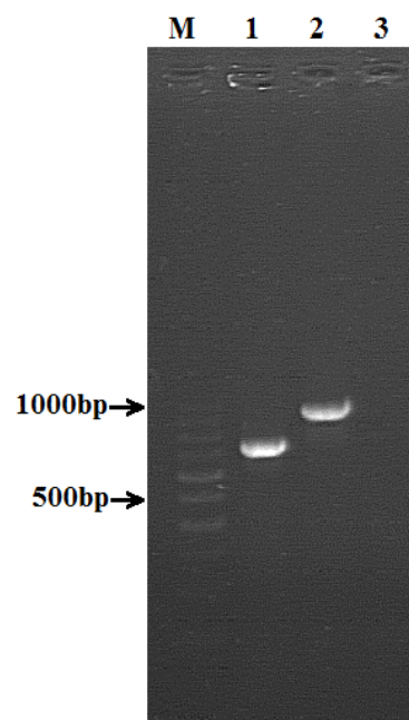
Figure 2. Diagnostic multiplex PCR using a combination of 3 primers in each reaction. Lane M: DNA size marker; Lane 1: T. urticae ; Lane 2: T. turkestan i, Lane 3: C - .
