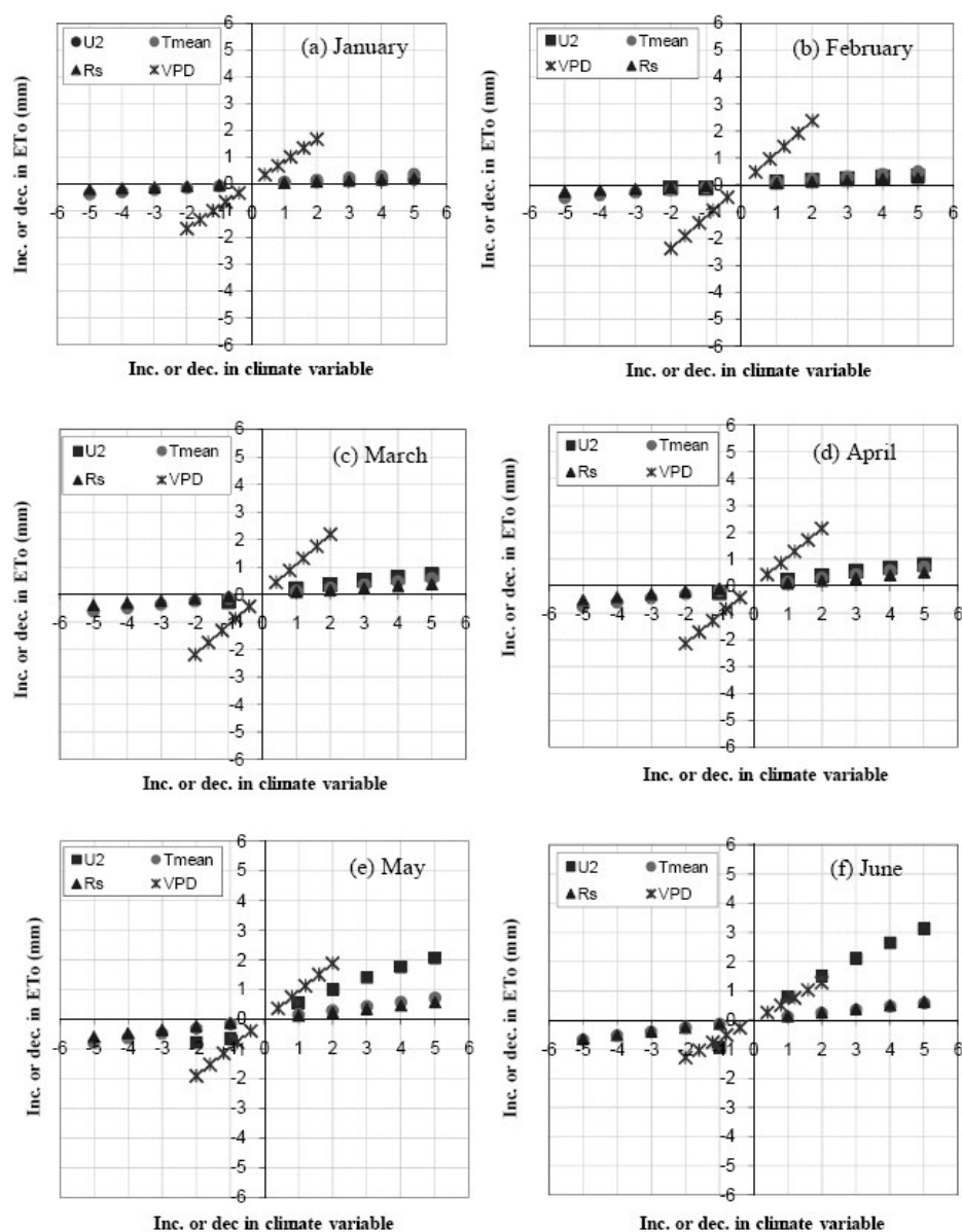
Figure 2. Changes in ET_0 (mm d^{-1} ) with respect to increase or decrease in four climatic variables ( T_{mean} is mean air temperature, VPD is vapor pressure deficit, U_2 is wind speed at 2 m and R_s is solar radiation).
