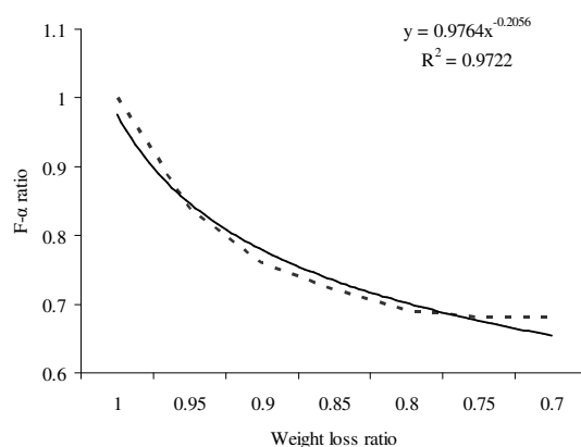
Figure 5. Relationships between weight loss ratio and F-\alpha ratio in Flame, using data from Figure 2.
