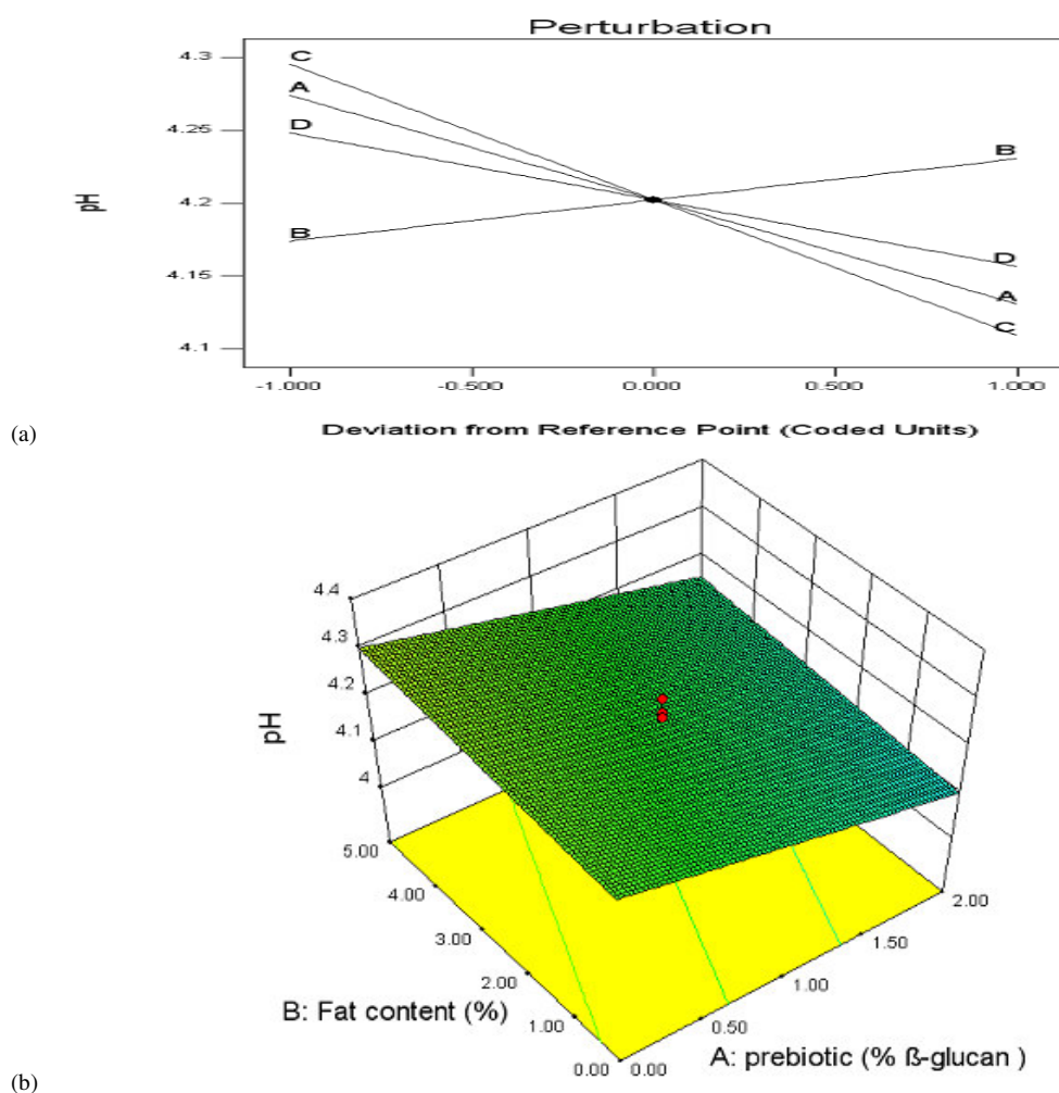
Figure 3. Effect of various factors on the rate of camel yogurt Ph: (a) Perturbation and (b) 3D graphs. A, B, C and D are prebiotic ( \beta -glucan) percentage, camel milk fat percentage, inoculated probiotic bacteria percentage and storage time, respectively.
