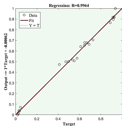
Figure 7. Analysis of the predicted vs. actual crop yield outputs using linear regression.
