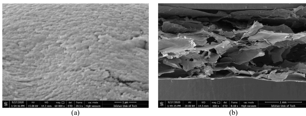
Figure 1. FE-SEM images of agar cryogel from (a) Surface and (b) Cross-section.
