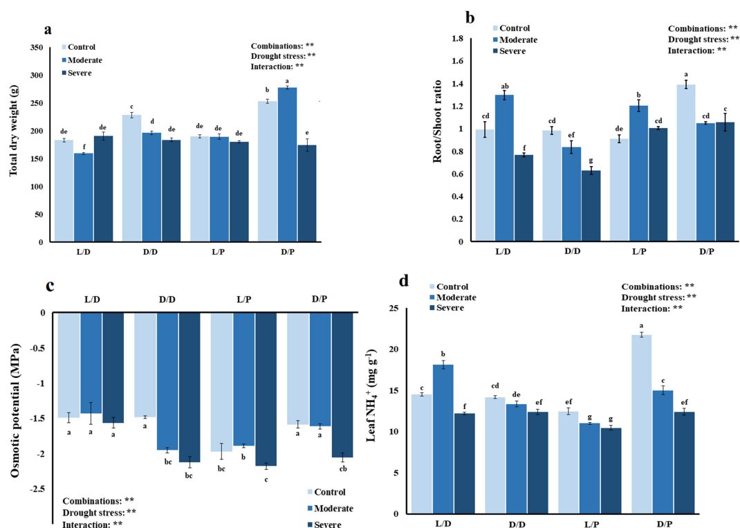
Figure 3. (a) Total Dry Weight (TDW), (b) Root-to-shoot ratio, (c) osmotic potential ( \Psi_s ), and (d) Leaf \text{NH}_4^+ of four scion-rootstock combinations (L/D: 'Louise Bonne'-'Dargazi', D/D: 'Dargazi'-'Dargazi', L/P: 'Louise Bonne'-'Pyrodwarf', D/P: 'Dargazi'-'Pyrodwarf') under three different drought stress conditions (control, moderate, severe). Vertical bars represent the \pm standard error of the mean ( n=4 ). Different letters above individual bars indicate statistically significant differences among treatments at P \leq 0.05 based on Duncan's multiple range test. ns, and **: Not significant, and significant at P \leq 0.01 , respectively.
