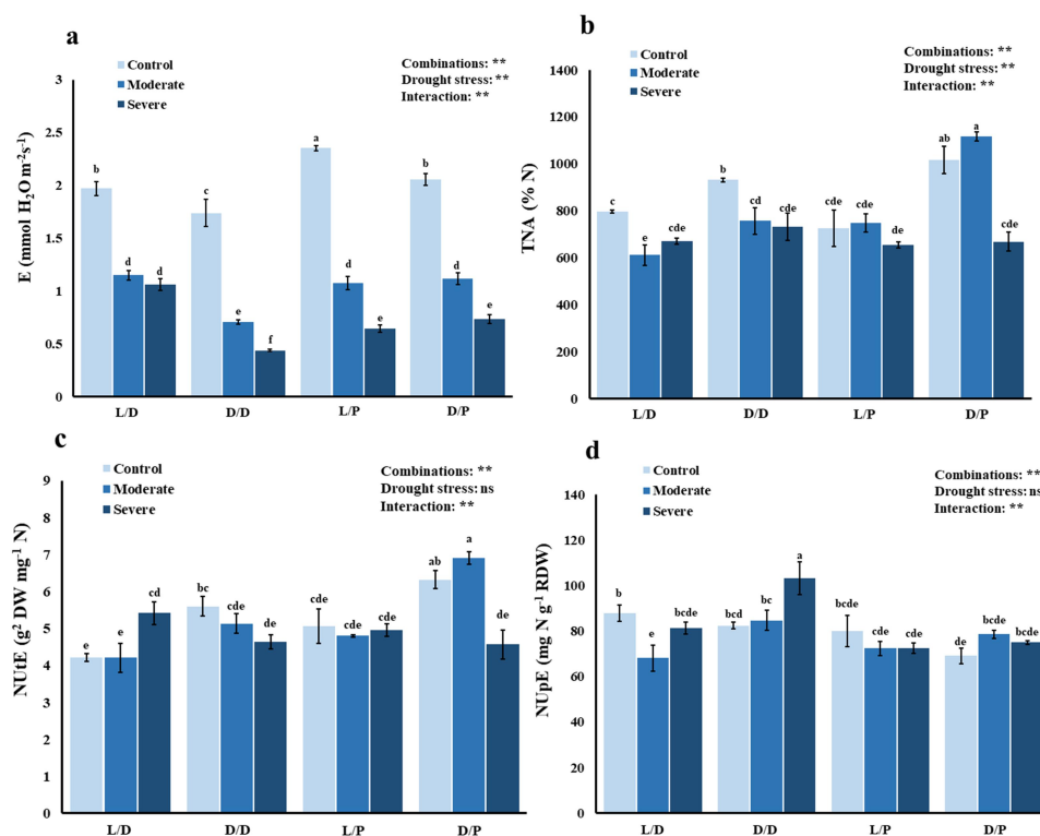
Figure 5. (a) Transpiration rate (E), (b) Total Nitrogen Accumulation (TNA), (c) Nitrogen Utilization Efficiency (NUE), and (d) Nitrogen Uptake Efficiency (NUpE) of four scion-rootstock combinations (L/D: 'Louise Bonne'-'Dargazi', D/D: 'Dargazi'-'Dargazi', L/P: 'Louise Bonne'-'Pyrodwarf', D/P: 'Dargazi'-'Pyrodwarf') under three different drought stress conditions (control, moderate, severe). Vertical bars represent the \pm standard error of the mean ( n=4 ). Different letters above individual bars indicate statistically significant differences among treatments at P \leq 0.05 based on Duncan's multiple range test. ns, and **: Not significant, and significant at P \leq 0.01 , respectively.
