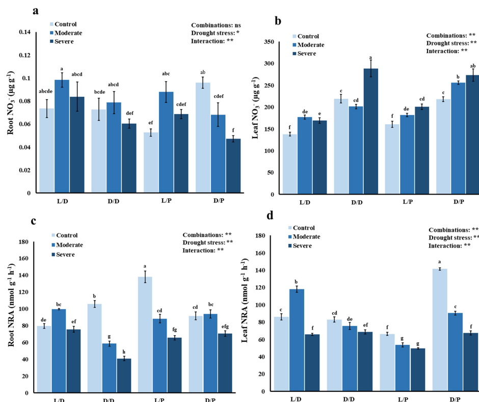
Figure 4. (a) Root \text{NO}_3^- , (b) Leaf \text{NO}_3^- , (c) Root nitrate reductase activity (NRA), and (d) Leaf nitrate reductase activity (NRA) of four scion-rootstock combinations (L/D: 'Louise Bonne'-'Dargazi', D/D: 'Dargazi'-'Dargazi', L/P: 'Louise Bonne'-'Pyrodwarf', D/P: 'Dargazi'-'Pyrodwarf') under three different drought stress conditions (control, moderate, severe). Vertical bars represent the \pm standard error of the mean ( n=4 ). Different letters above individual bars indicate statistically significant differences among treatments at P \leq 0.05 based on Duncan's multiple range test. ns, *, and **: Not significant, significant at P \leq 0.05 and P \leq 0.01 , respectively.
