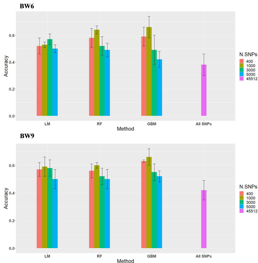
Figure 4. Accuracy of genomic prediction of all SNPs and different subsets of using a 5-fold cross-validation approach for BW6 and BW9 from LM, RF and GBM methods.
