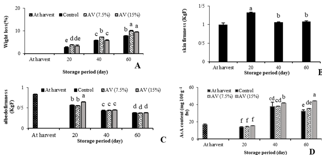
Figure 1. Effect of AV gel treatments and storage time on weight loss (A), peel (B), and pulp (C) firmness and vitamin C (D) of lime fruit stored at 4\pm1^{\circ}\text{C} , 85\pm2\% RH. Vertical bars indicate the standard errors of 4 replicates. Values with similar letters are not significantly different ( P\leq 0.05 ).
