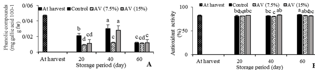
Figure 4. Effect of AV gel treatments and storage time on phenolic compounds and antioxidant activities of lime fruit stored at 4 \pm 1^\circ\text{C} , 85 \pm 2\% RH. Vertical bars indicate the standard errors of 4 replicates. Values with similar letters are not significantly different ( P \leq 0.05 ).
