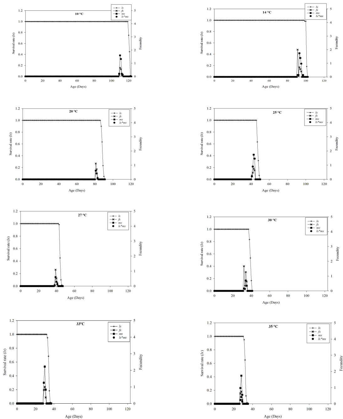
Figure 2. Age-specific survival rate ( l_x ), age-specific fertility ( f_x ), fertility ( m_x ), and age-specific maternity ( l_x \cdot m_x ) of the carob moth ( E. ceratoniae ), at different temperatures in the laboratory.
