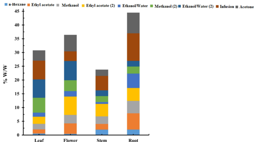
Figure 5. Extraction yield of different solvent from different organs of D. ammoniacum .
