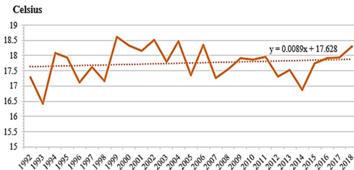
Figure 3. Temperature trend in Bakhtegan-Tashk Basin (IMO, 2019).
