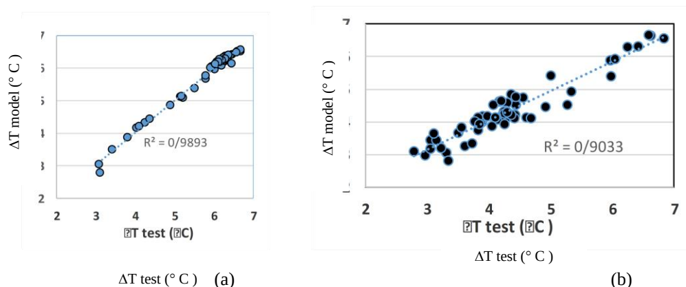
Figure 6. Comparison of temperature drops from the model and experimental data: (a) FPS and (b) IDEC system.
