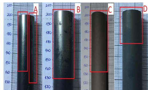
Figure 5. Second-speed wear appearance on coated teeth.
