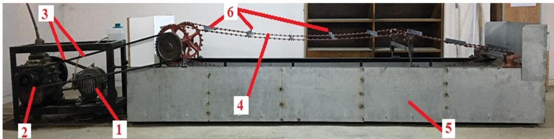
Figure 1. Sample wear pattern: (1) Electric motor, (2) Gear box, (3) Belt-pulley, (4) Gal type chain, (5) Wear bin, (6) Assembly points.
