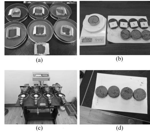
Figure 3. Test experiment of soil parameters: (a) Screening method to measure the distribution of soil particle size; (b) Ring knife method to measure soil bulk density; (c) ZJ strain control direct shear, (d) Direct shear test.
