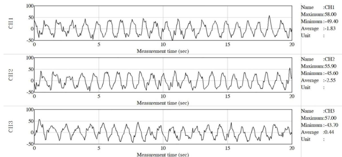
Figure 13. Variation of strain with time at the measuring points 1, 3, and 5.
