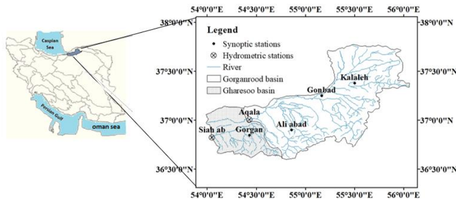
Figure 1. Location of selected synoptic and hydrometric stations in the study basin.
