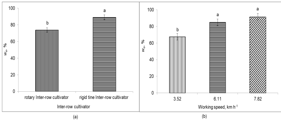
Figure 7. Effects of different inter-row cultivators and working speeds on Weeding efficiency (We). Means followed by different lower-case letters are significantly different according to LSD's multiple range test at the significance level of 0.05; error bars are standard errors.
