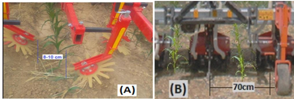
Figure 1. Modified hoeing equipment for strip tillage applications (A) and hoeing equipment with a rotary tiller (B).
