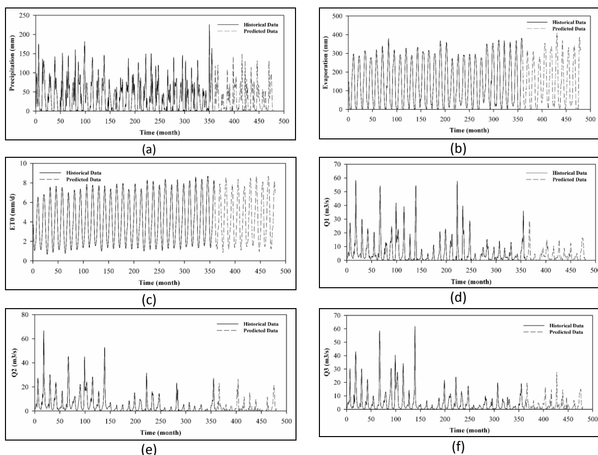
Figure 4. Variations in historical and (a) Predicted precipitation; (b) Predicted evaporation; (c) Predicted potential Evapotranspiration (ET0); (d) Predicted Q1; (e) Predicted Q2 and, (f) Predicted Q3 over a period of 480 months. "Q1, Q2 and Q3" are river discharge in three hydrometry stations in the study area.
