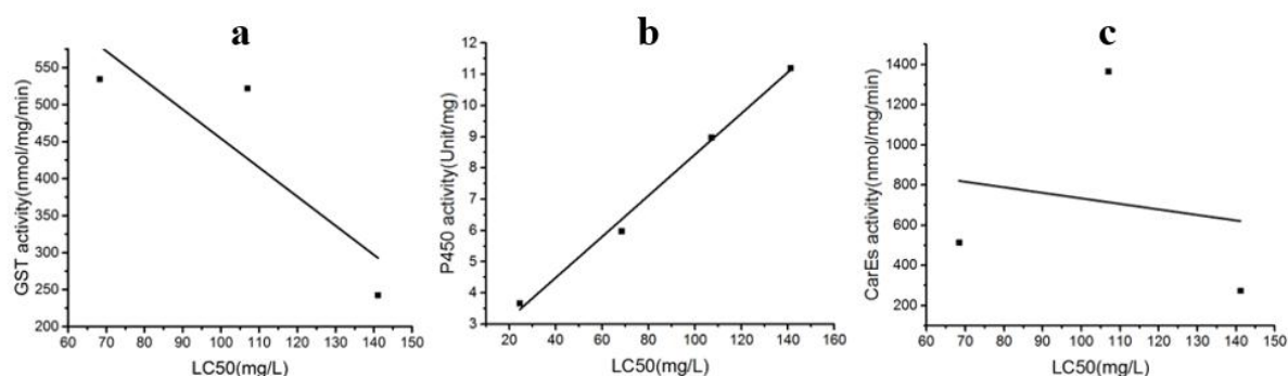
Figure 2. Correlation between the LC 50 values of the populations and activity of detoxification enzymes. Pearson's r: -0.87 (a), 0.99 (b) and -0.17 (c).
