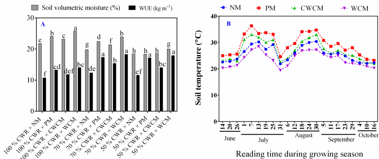
Figure 2. Effect of irrigation regimes and mulch treatments on water use efficiency and soil temperature and moisture. Symbols are defined in the text and Figure 1. Values followed by different letters are significantly different ( P < 0.05 ; Tukey's least significant difference test; n = 3 ).
