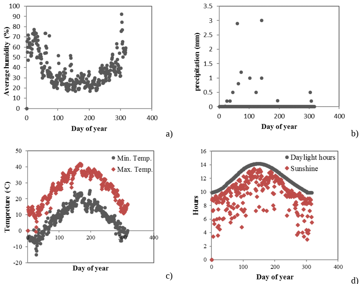
Figure 4. Daily evolution of: (a) Average humidity; (b) Precipitation; (c) Minimum and maximum temprature, and (d) Dalight hours and sunshine duration in 2001 to represent how they change during a typical year in this region.
