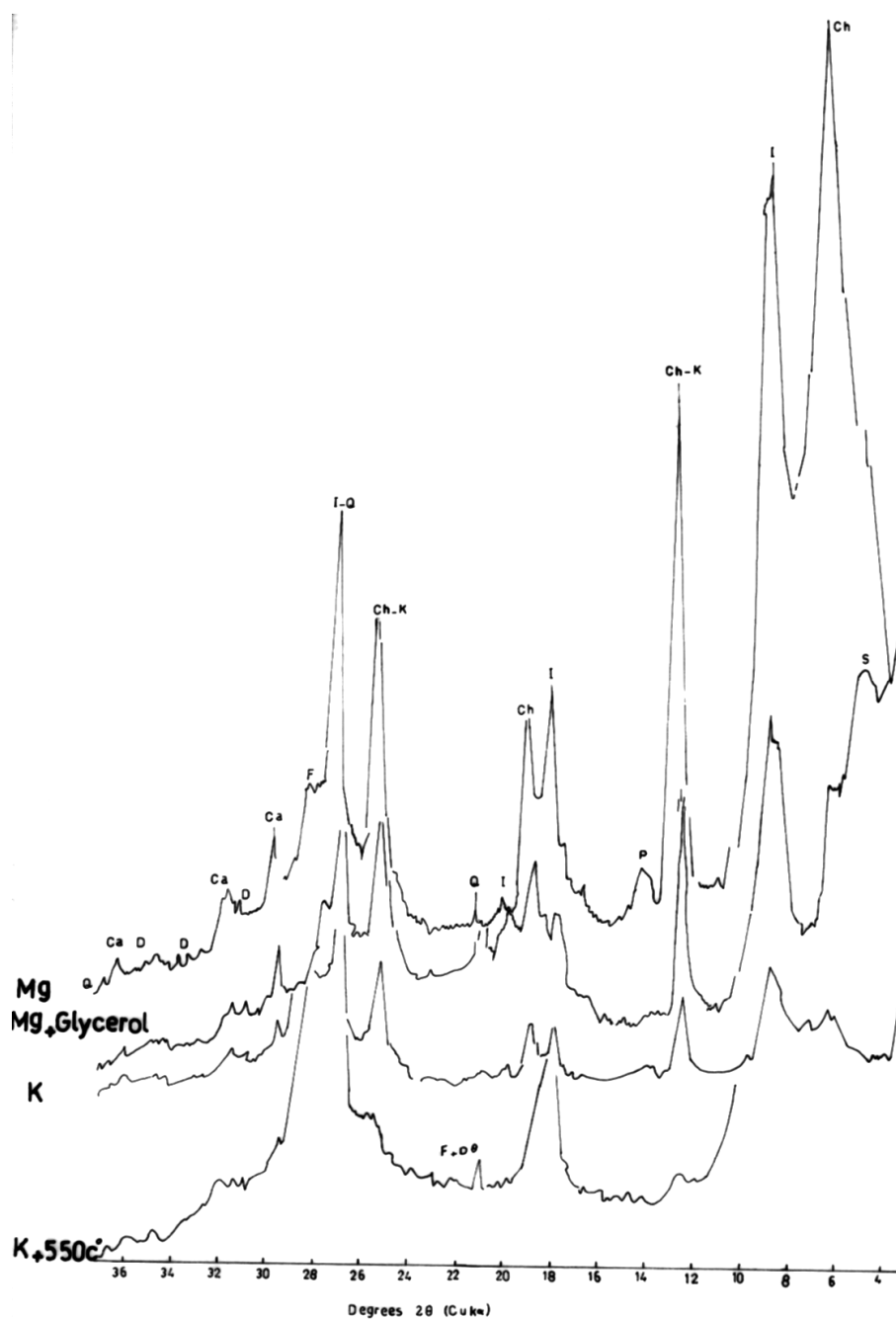
Figure 3. XRD patterns for the < 2 \mu\text{m} fraction of the treated alluvium from the first sedimentation basin. Ca:calcite; Ch:chlorite; D: dolomite, F: alkali feldspars; S:smectite. I: illite; K:kaolinite; P:plagioclase; Q: quartz
