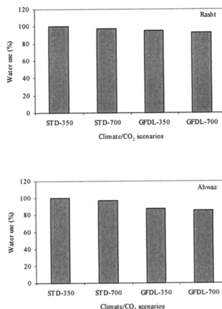
Figure 5. Effect of climate/CO 2 scenarios on crop water use (as a percent of current conditions) in Rasht and Ahwaz. Simulated crop water use are 408 and 1327 mm under current climate/CO 2 for Rasht and Ahwaz, respectively. STD and GFDL are the current and Geophysical Fluid Dynamics Laboratory climates, respectively.
