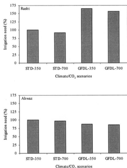
Figure 6. Effect of climate/CO 2 scenarios on irrigation needs (as a percent of current conditions) in Rasht and Ahwaz. Simulated irrigation need are 127 and 1319 mm under current climate/CO 2 for Rasht and Ahwaz, respectively. STD and GFDL are current and Geophysical Fluid Dynamics Laboratory climates, respectively.
