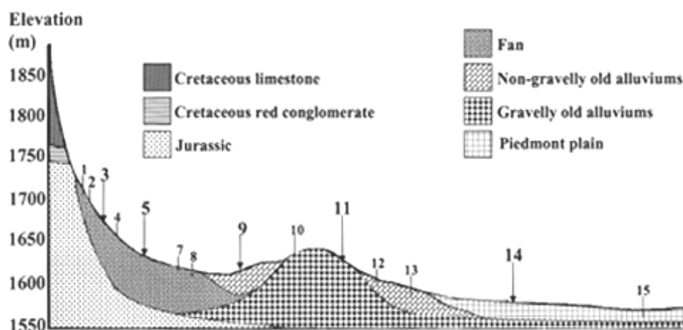
Figure 2. Cross-section showing the geology and landforms in study area.
