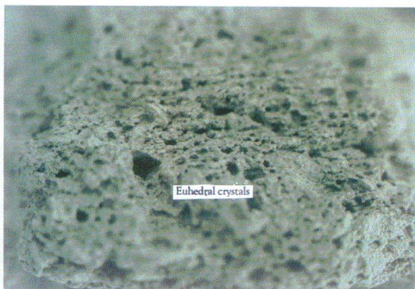
Figure 6. Vesicular soil crust, formed under desert pavement on surface of profile No. Eleven (Hand specimen).
