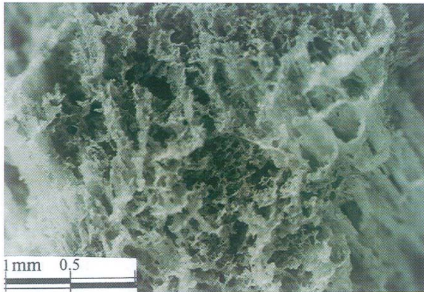
Figure 7. Changing the arrangement of gypsum crystals in 2Y3 horizon of profile No. Eleven (Hand specimen).
