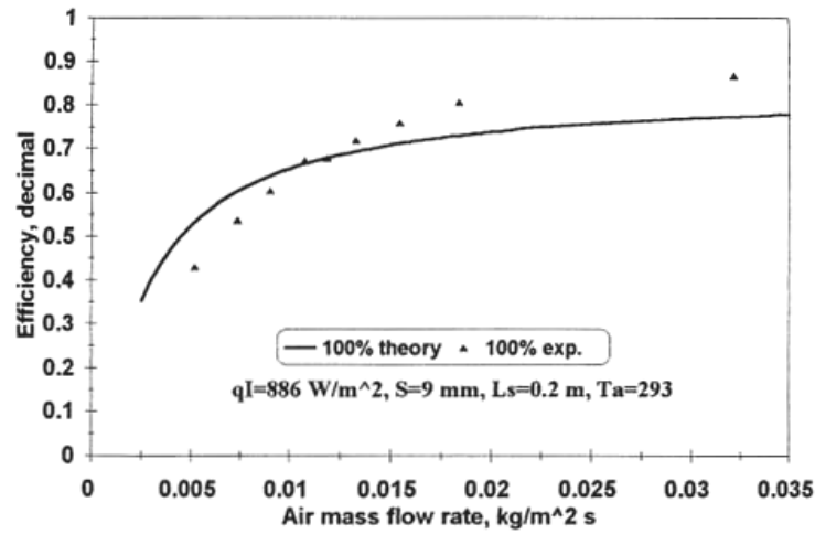
Figure 6. The relationship between air mass flow rate and absorber efficiency for 100% models (theoretical and experimental values).
