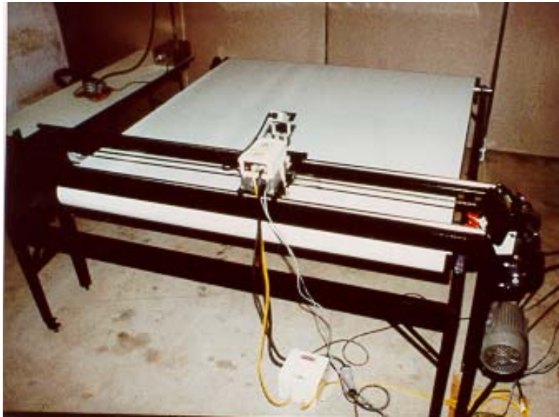
Figure 2. An experimental prototype of the simulator.
