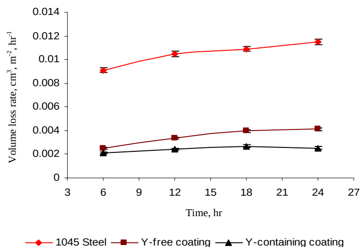
Figure 7. Volume loss of the aluminide coatings with and without yttrium, and 1045 steel (slurry erosion test machine).
