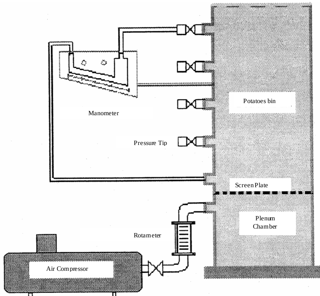
Figure 1. Schematic diagram of the apparatus for measuring the airflow resistance of potatoes.
