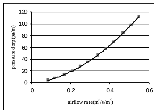
Figure 2. A typical curve of resistance of potatoes to airflow.
