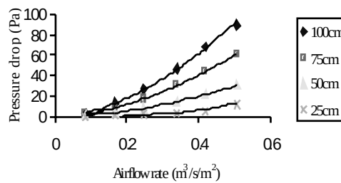
Figure 4. Airflow resistance of potatoes at different bed depths.
