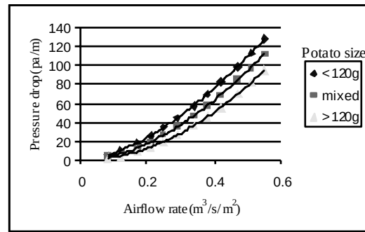
Figure 3. Airflow resistance for different potato sizes.
