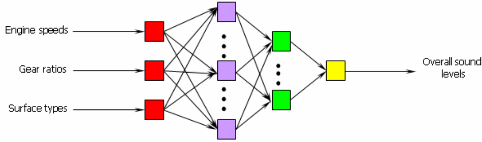
Figure 4. Topology of the artificial neural network.
