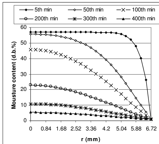
Figure 6. Moisture distribution at selected drying times for a pistachio nut (1/4 kernel shown) at initial moisture content of 56.9 (d.b.%) and T= 70\text{ }^{\circ}\text{C} .
