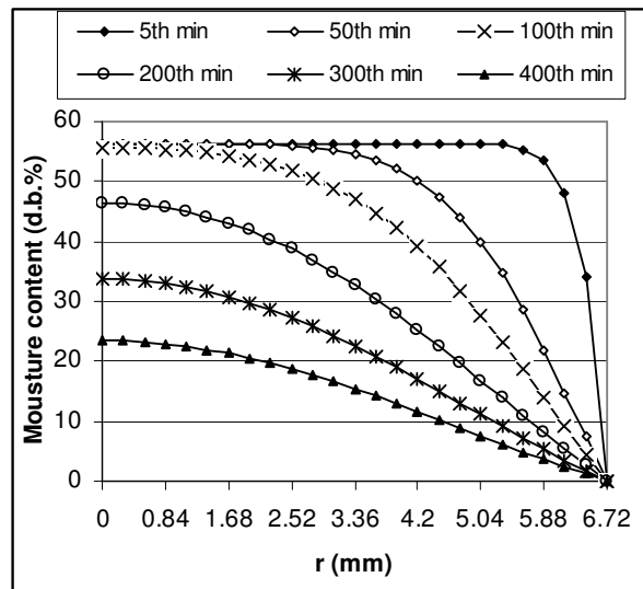
Figure 5. Moisture distribution at selected drying times for a pistachio nut (1/4 kernel shown) at initial moisture content of 56.3 (d.b.%) and T= 55\text{ }^{\circ}\text{C} .
