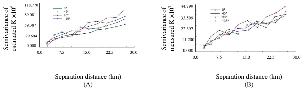
Figure 4. Experimental semi-variograms of the estimated (A) and measured (B) soil erodibility factors in the study area in the different directions.
