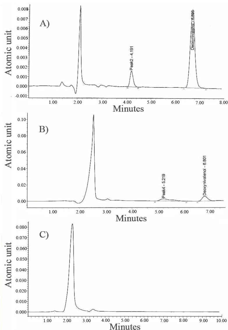
Figure 1. HPLC chromatograms of (A) Deoxynivalenol standard 1000 ng ml -1 , (B) Corn spiked sample with 1.0 ppm (C) Blank corn sample. HPLC condition, column: 250×3.9 mm, C18 reverse phase ODS, 4 µm; mobile phase: acetonitrile: water (1:9; v/v); flow rate: 1.0 ml min -1 ; UV detector: 218 nm.
