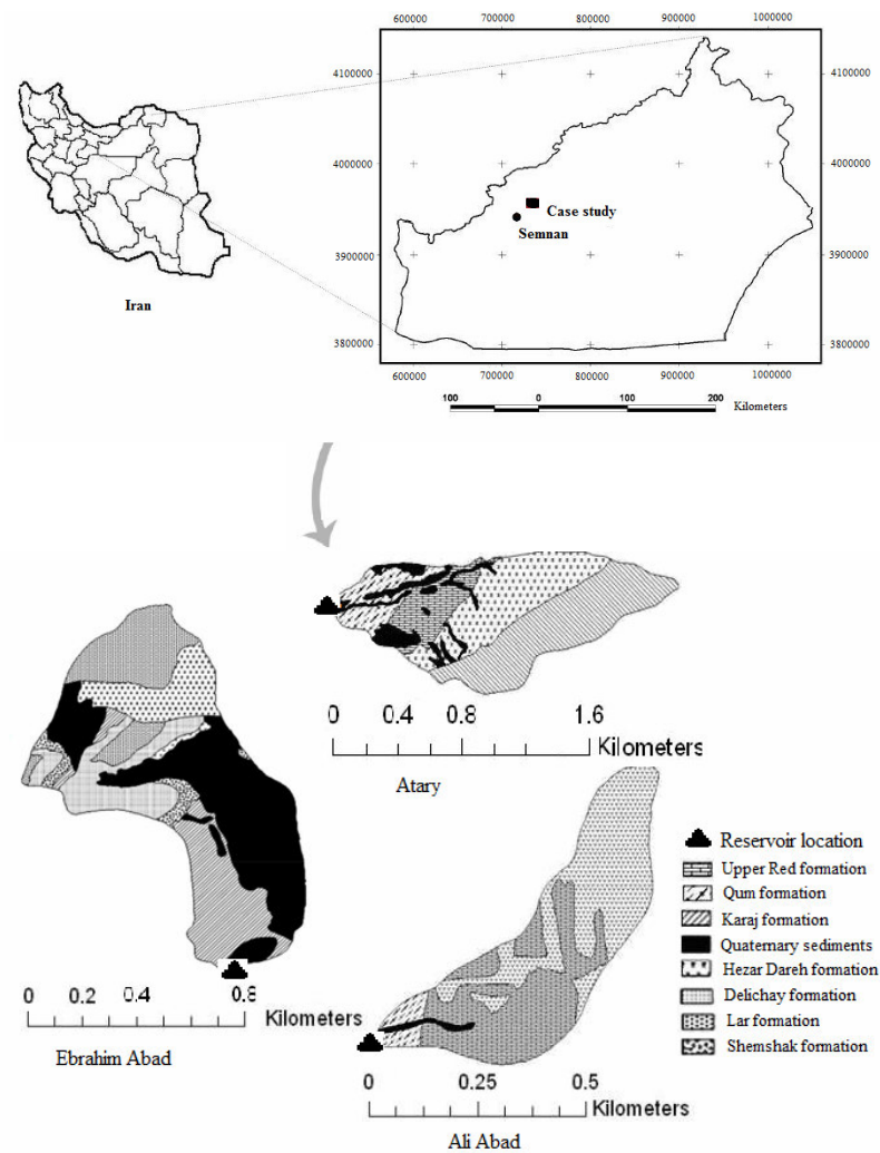
Figure 1. Location map of the study area and the geological formations of each study catchment basin.
