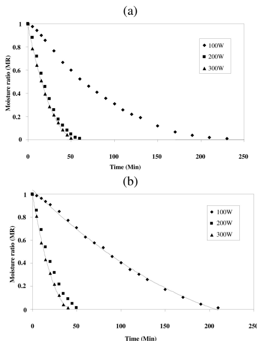
Figure 5. Moisture ratio data for sweet (a) and sour (b) pomegranate arils at various operating powers in the microwave drier along with the curves predicted by the Midili model.
