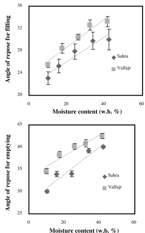
Figure 7. Effect of moisture content on angle of repose of barley kernels.
