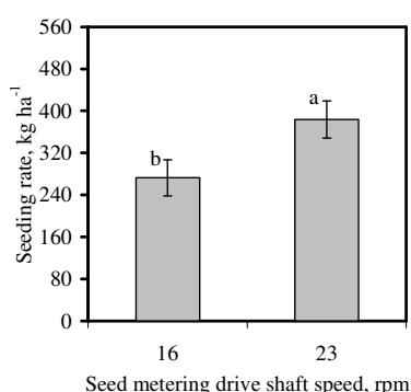
Figure 2. Effect of seed meter drive shaft speed on wheat seeding rate (the test rig speed was 3.6 km h -1 ). Vertical bars indicate \pm 1 standard deviation of the mean. Columns with different letters differ at P < 0.05 as tested by Duncan multiple range test.
