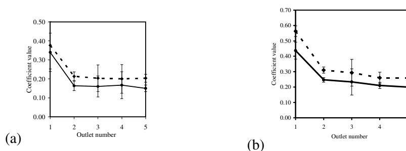
Figure 9. Comparison of coefficient of variation (CV; \text{---}\blacklozenge\text{---} ) and non-uniformity coefficient ( 1-U_c ; \text{---}\bullet\text{---} ) for the seed meter drive shaft speed of a) 23 rpm, and b) 16 rpm for wheat. (The test rig speed was 3.6 \text{ km h}^{-1} ). Vertical bars indicate \pm 1 standard deviation of the mean.
