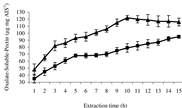
Figure 1. Extraction curve of oxalate-soluble pectin concentration of Asian pear ('KS' 13 ) extracted through hot water ( 95\pm 2^{\circ}\text{C} ). Data are the means (3 fruits) with the error bar indicating the standard error.
