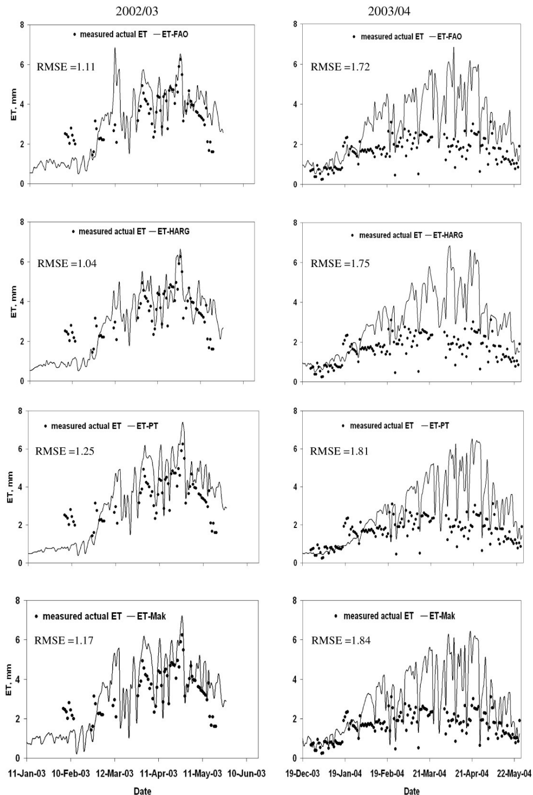
Figure 3. Comparison between daily evapotranspiration measured by eddy covariance technique and the estimated one ( ET = K_c \times ET_0 ) using different methods for estimation ET_0 and the crop coefficients proposed by the FAO-56 (Allen et al. , 1998) for winter wheat during 2002/03 and 2003/04 growing seasons.
