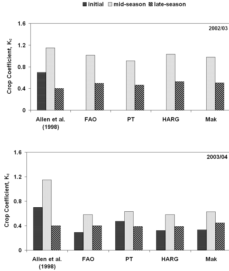
Figure 5. Estimated crop coefficients for winter wheat at three growth stages by different climatological methods for estimating ET_0 with the standard values recommended by Allen et al. (1998) in two growing seasons: 2002/03 and 2003/04. No values of crop coefficient are shown during the initial stage in 2002/03 due to the missing of evapotranspiration measurement (see Figure 2).
