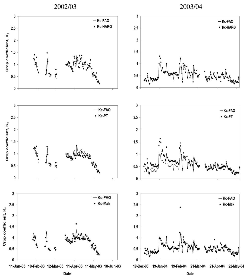
Figure 4. Seasonal changes in crop coefficient estimated as the ratio of the measured ET and the ET_0 estimated by different methods using meteorological data for winter wheat during 2002/03 and 2003/04 growing seasons.
