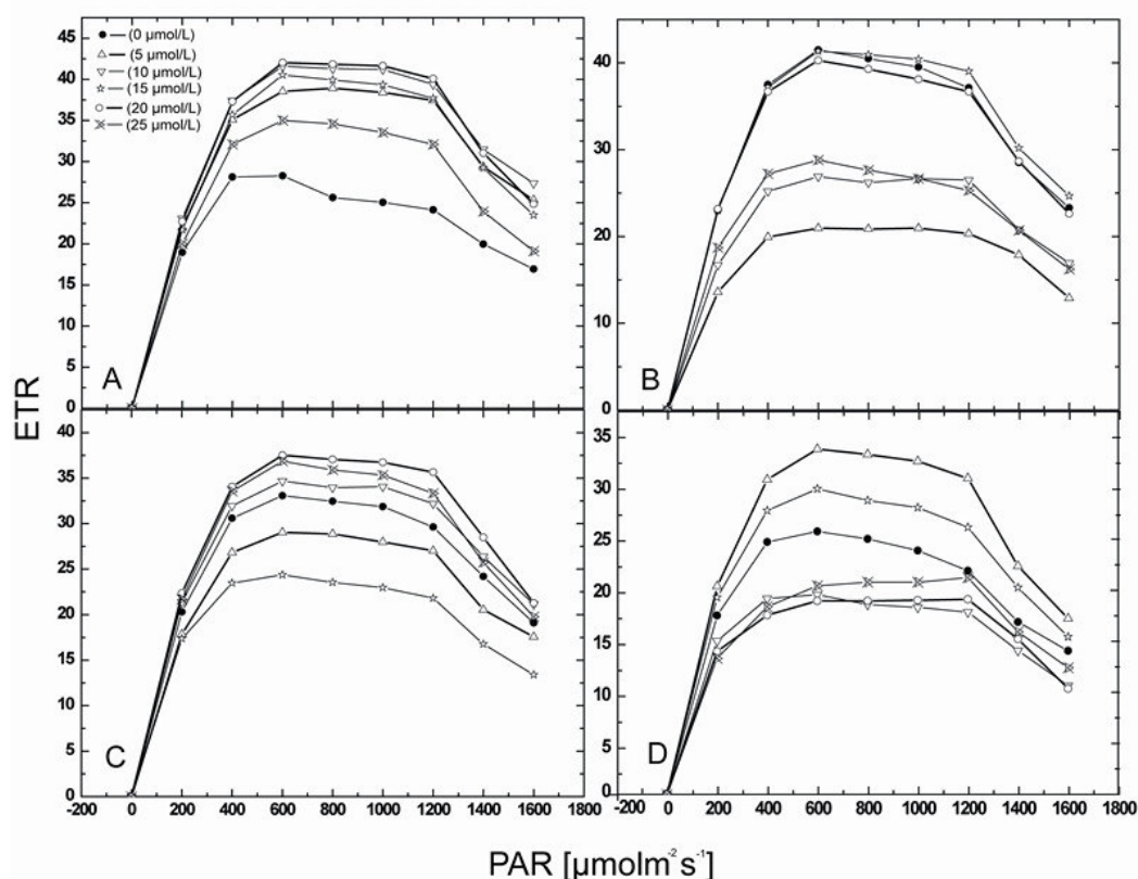
Figure 7. Changes in apparent electron transport rate ( ETR ) in response to light irradiance at different levels of zinc treatments under the salt concentrations of 0 (A); 100 (B); 200 (C), and 300 mmol L -1 (D).
