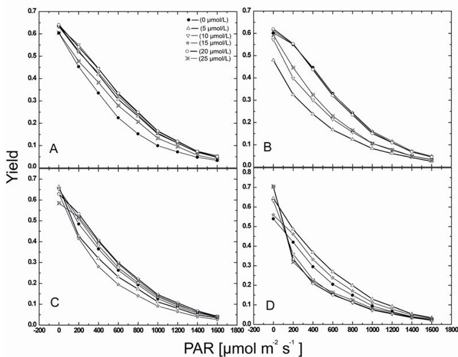
Figure 6. Changes in photochemical energy conversion (yield) in response to light irradiance at different levels of zinc treatments under the salt concentrations of 0 (A); 100 (B); 200 (C), and 300 mmol L -1 (D).
