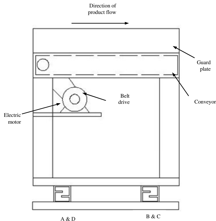
Figure 9. Schematic diagram of the load cell supporting system.
