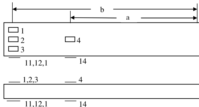
Figure 1. Positioning strain gauges on the beams.
