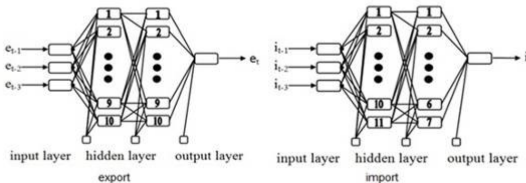
Figure 1. The ANN architecture selected for the prediction model regarding export and import.
