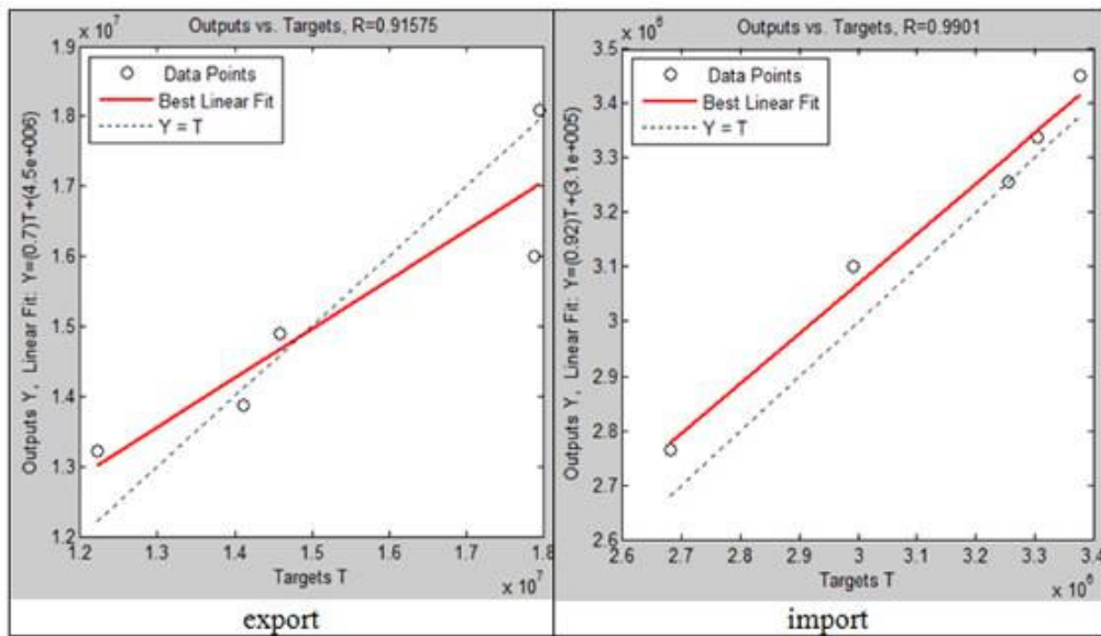
Figure 3. Relation between the real values and the ANN values.
