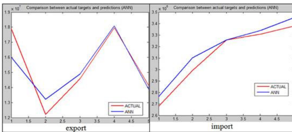
Figure 4. Comparison of the real values with the ANN values.
