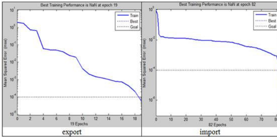
Figure 2. Iteration dependant error variation graphics of the ANN.
